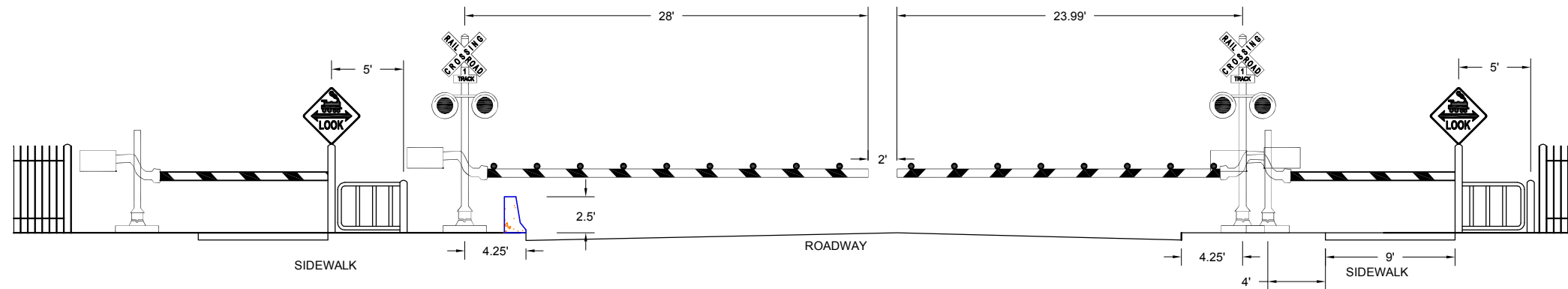
SECTION B-B
