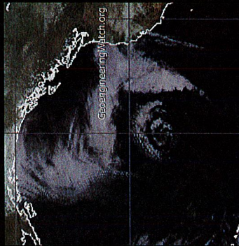
NOAA satellite image, radio frequency / microwave transmission manipulation of Eastern Pacific storm system. GeoengineeringWatch.org
